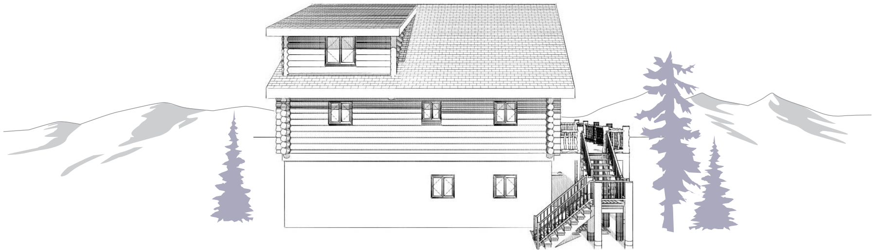
LEFT ELEVATION
